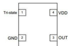
Pin Assignments
