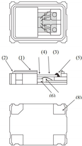
Figure 4. Internal Structure
