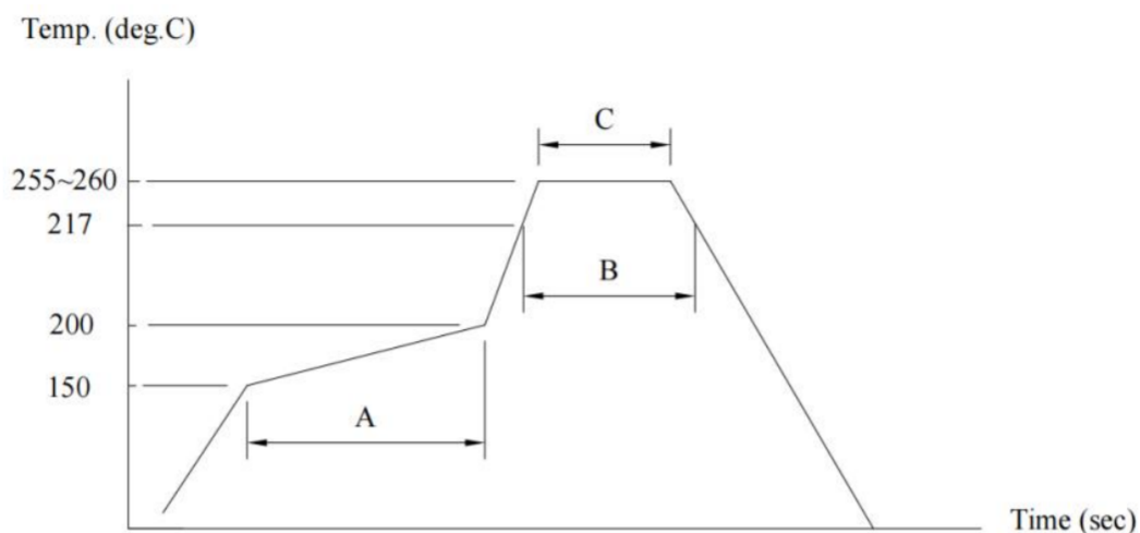
Figure 5. Reflow Profile
