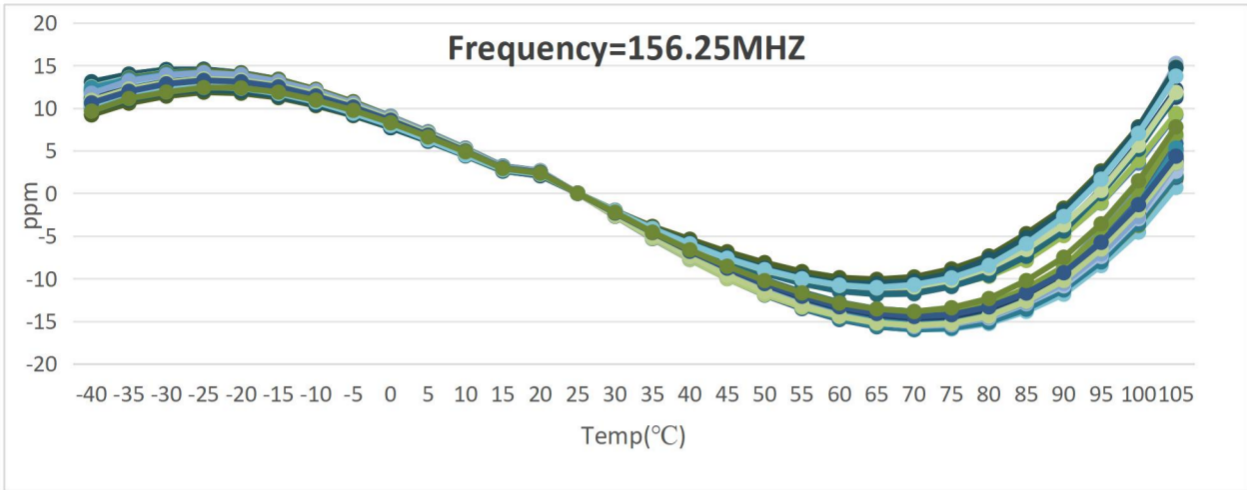
Figure 2 Frequency vsTemperature
