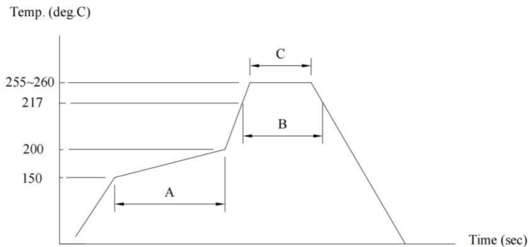
Figure 4. Reflow Profile
