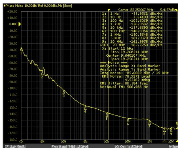
Figure 1 Representative Phase Noise Measurement
