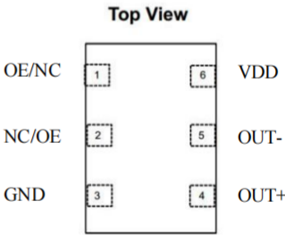
Figure 3 Pin Assignments
