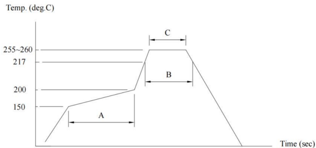
Figure 6. Reflow Profile
