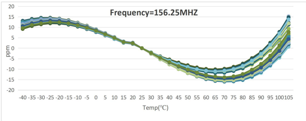
Figure 4 Frequency vsTemperature
