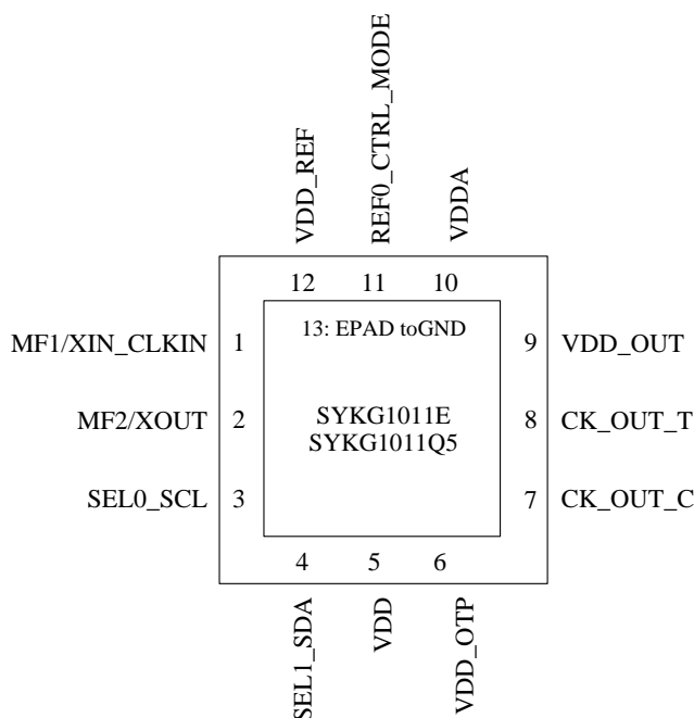
Figure 2. 12-LGA Pin Assignment, 2.5mm x 2.5mm x 1.1mm, 0.5mm Pitch (Top view)
