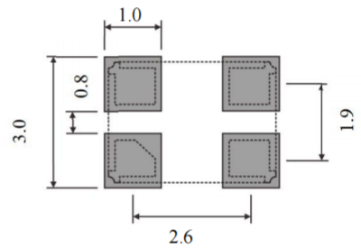
Recommended soldering Pattern
